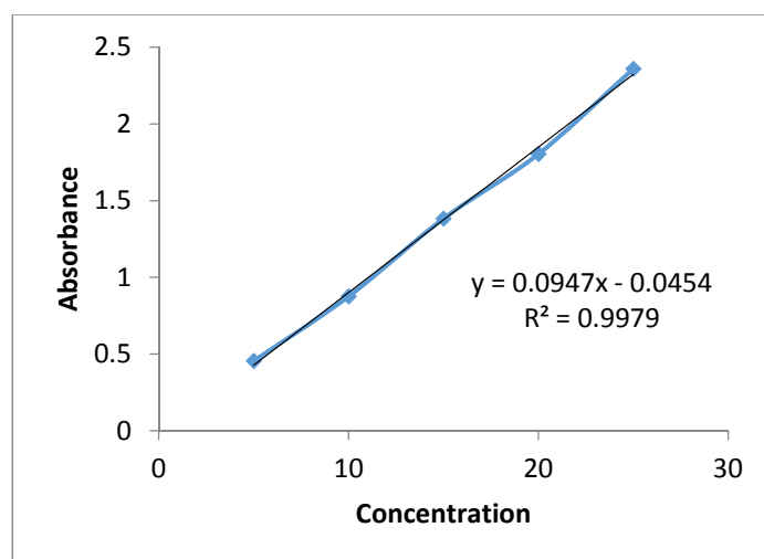
Fig. 4 calibration curve of hydrochlorothiazide
