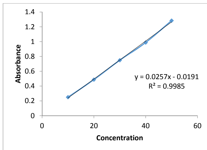
Fig. 3 calibration curve of propranolol hydrochloride
