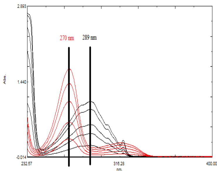
Fig. 2 Overlain linear zero order spectra of PRO (Red) and HCT (Black) in 2:1 ratio
