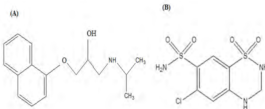
Fig.1 (A) is Structure of propranolol hydrochloride and (B) is structure of Hydrochlorothiazide.
